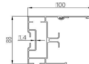
Guide rail
